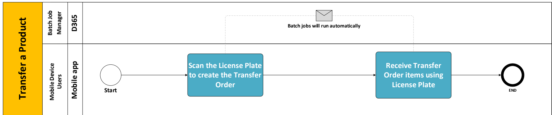
Figure 1 Process Flow Map (To-Be)
